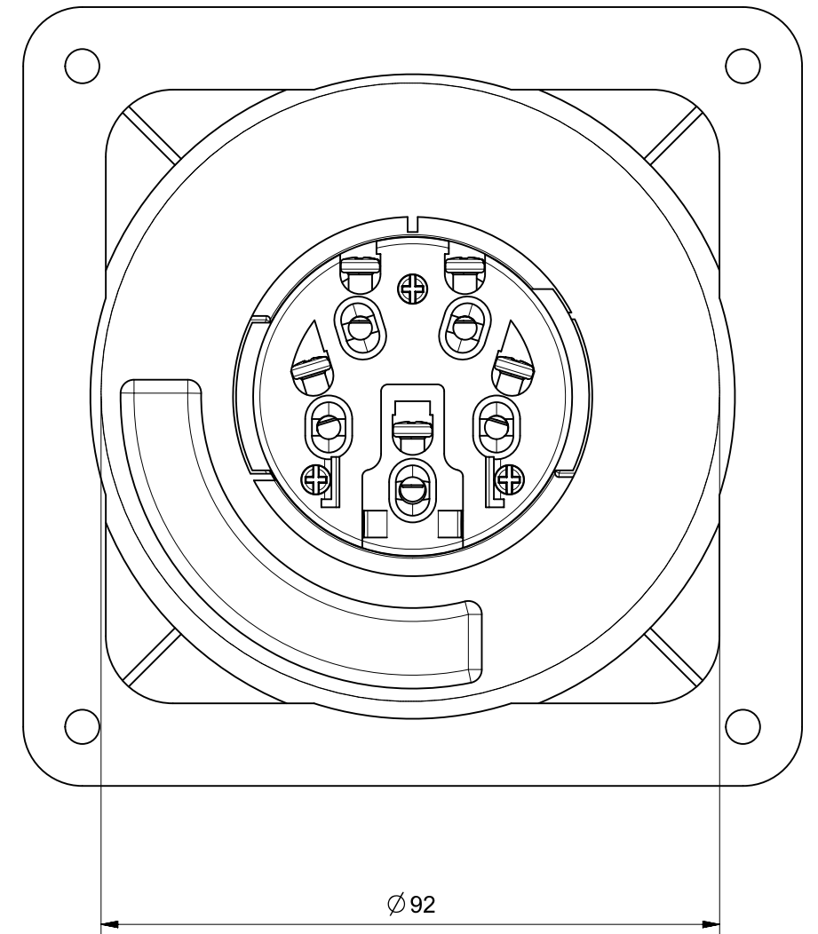
FORATURA PANNELLO // PANEL DRILLING HOLE
