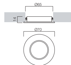
RECESSED MOUNTING
