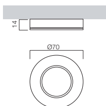
SURFACE MOUNTING
