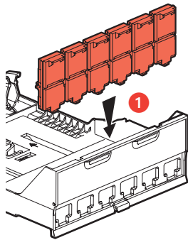
On cassette with 6 ports 0 337 55
