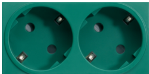
Priza dubla SCHUKO 45 mm, 16A, 230V, verde, 4M QC
