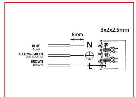
6. Leiter in die Klemme anschliessen / connect cable into the terminal block
