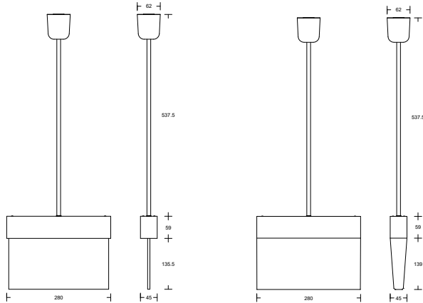
NLK1P105 + NLK2U013SC
