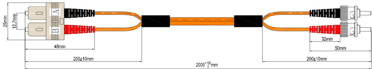
Dimensional drawing (example of 29021102)
