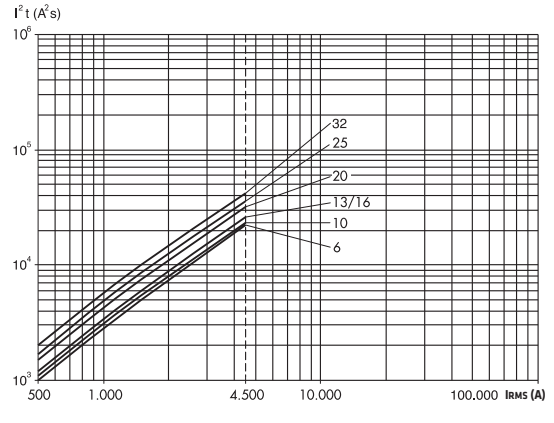
MTC 45 - 1P - 230V and 3P,4P - 230/400V versions
