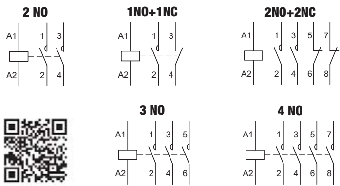
THK3-32, 3-40, 4-32, 4-40, 4-63
