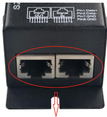
Port for sync-work signal
