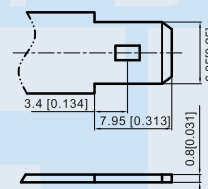
F2 (T2) terminal 6,35mm
