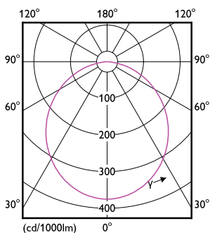
Downlight DN065C G3 LDNR 840 D225 RD-LDD
