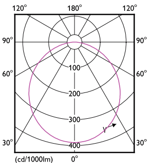
Downlight DN065B G3 LDNR 840 D150 RD-LDD
