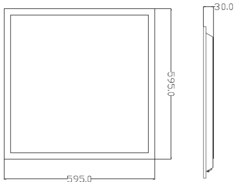
Diagrama dimensionala:
