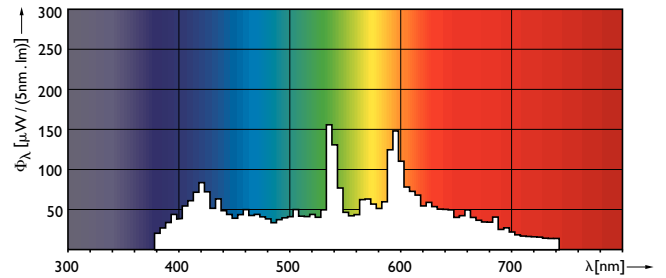
MASTERColour CDM-T 35W /842
