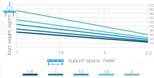
H: 50 - Perforated Cable Tray Load Graph
