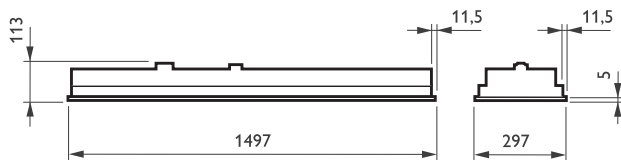
TBS461 2x35W/840 HFD ND AC-MLO W
