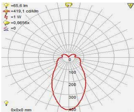
Photometric Diagram
