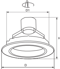
Legend: D - Outer diameter H - Height of the downlight D1 - Diameter of the cut
