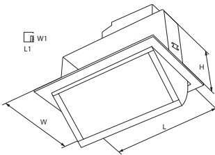
Legend: L/W - Outer size H - Height of the downlight L1/W1 - Size of the cut
