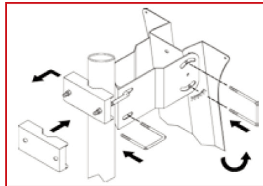
Fast mounting by U-bolt
