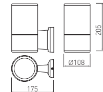
LD-BALGU10-0S
