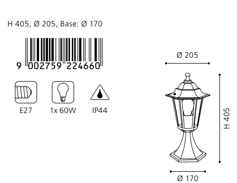
pedestal luminaire; cast aluminium, white / glass, clear Sockelleuchte; Aluguss, weiss / Glas, klar borne; aluminium moulé, blanc / verre, clair
