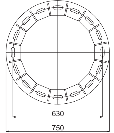
BASE PLATE t=20mm
