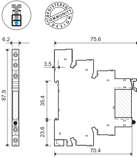
Tipurile 38.21 38.51/38.51.3 38.81/38.81.3 Terminal cu șurub
