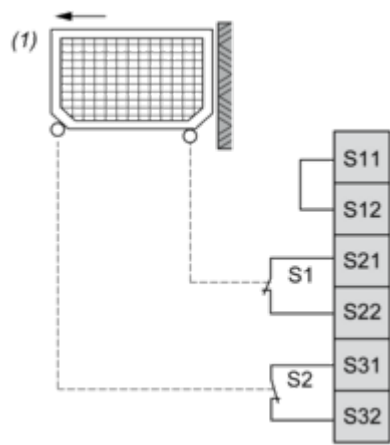
(1) Protective guard
