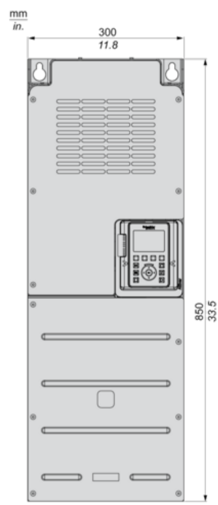
Drives with Lower Conduit Box Sold Separately Rear, Front and Left Views
