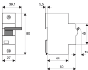
Shunt release
