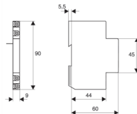
Auxiliary contact
