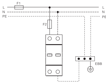
TN-S Network - Single-phase, 2+0 (T-connection)
