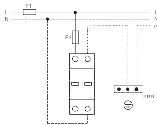
TT Network - Single-phase 1+1 (T-connection)
