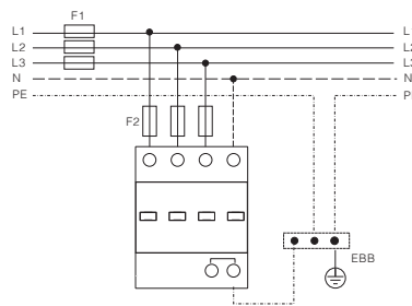
TN-S Network - Three-phase, 4+0 (T-connection)
