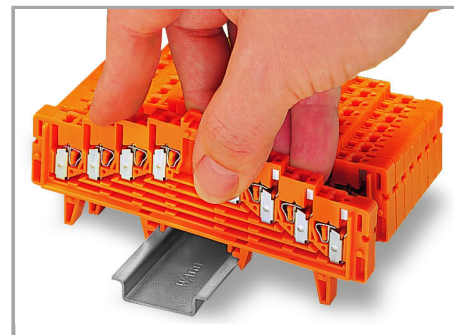
Snap individual 4- or 8-level terminal blocks onto the carrier rail.
