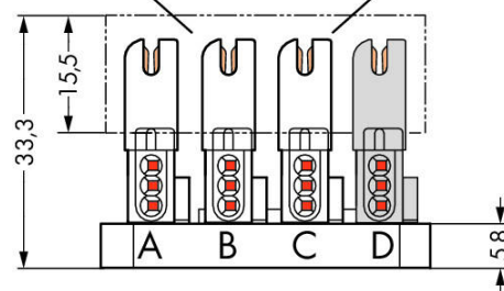
Snap-on type conductor support Socket module
