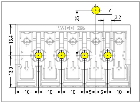
5-pole –with snap-in ground contact, d = 4.9 mm
