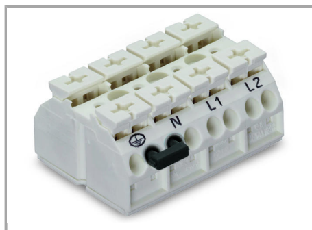
Commoning using a comb-style jumper bar (862-482).
