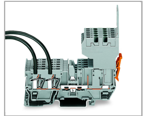
2-conductor female plug
