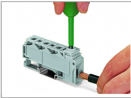
Terminating a 35 mm 2 (2 AWG) conductor –
