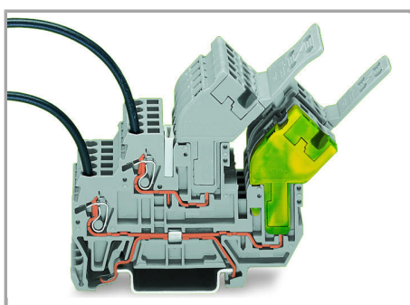
Angled female plugs provide reduced installation height.
