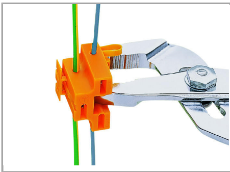
Press into final position using pliers.
