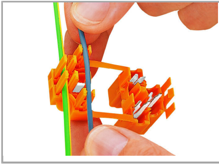
Press conductor into strain relief fingers.
