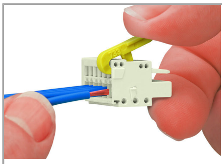
Inserting a conductor via 733-191 Operating Lever.
