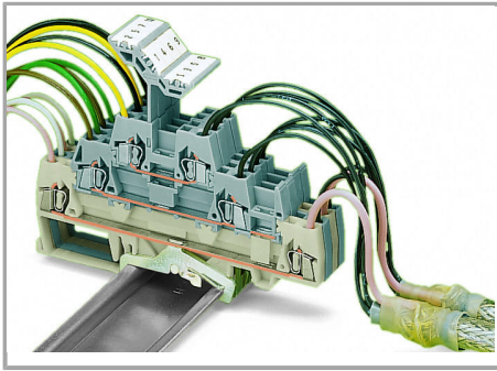
Shielded twisted pair cables
