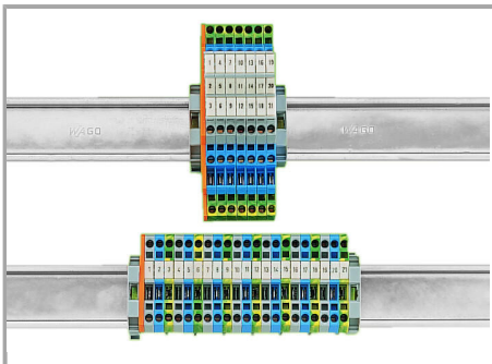
Save 67 % of rail space via triple-deck terminal blocks.
