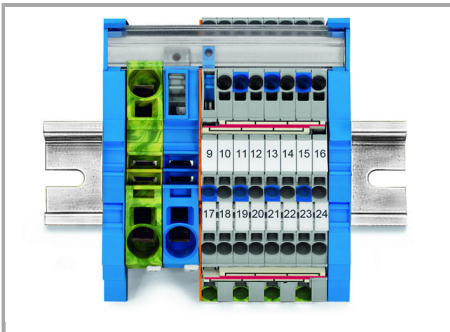
Mounting busbars on busbar carriers: Insert busbar ends onto large busbar carriers (2009-305) or onto supply terminal blocks (2009-305) or onto supply terminal blocks with an integrated busbar carrier.
