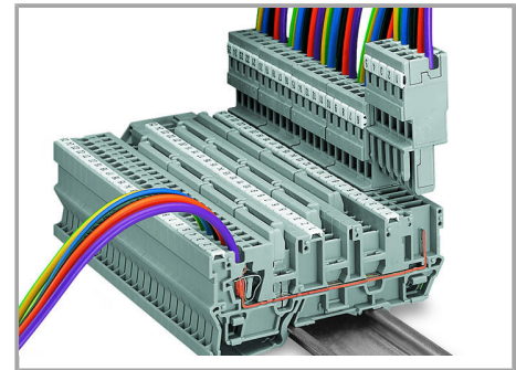
1-conductor/1-pin carrier terminal block with three jumper positions
