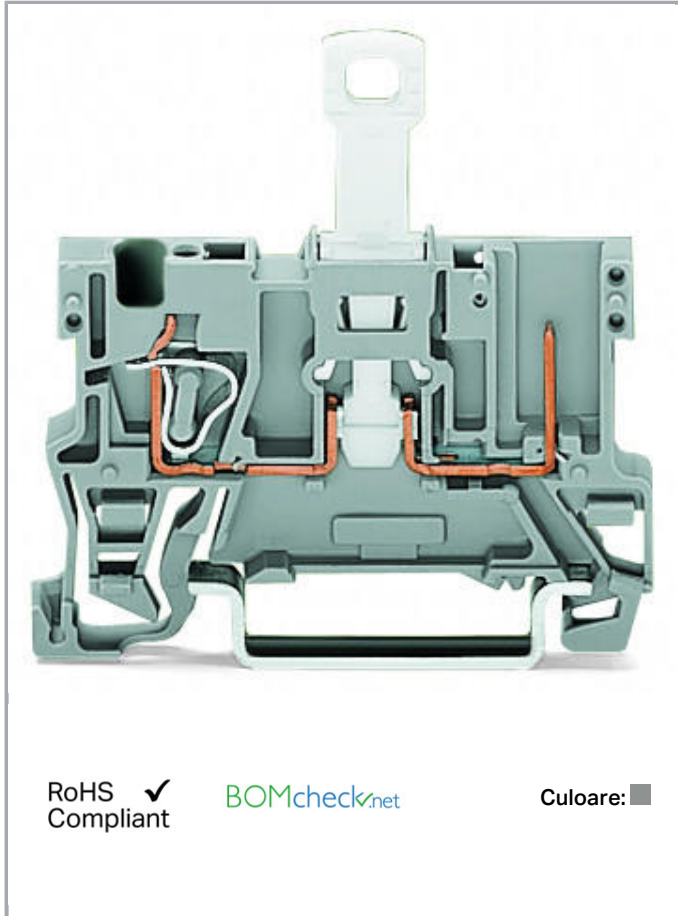
Disconnect carrier terminal block with shield contact
