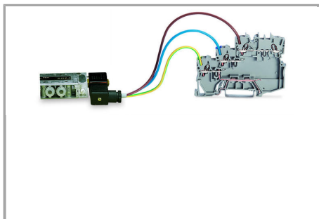
3-conductor actuator LED terminal block with a connected actuator
