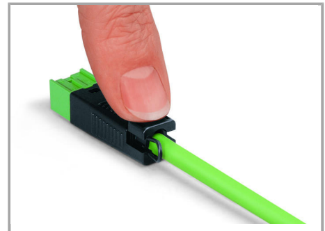
Press strain relief firmly on the cable.
