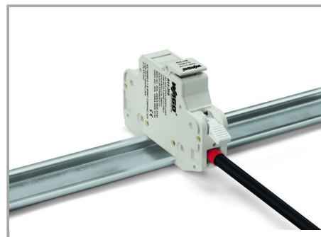
Terminating ferruled conductors up to 10 mm 2 (8 AWG).
