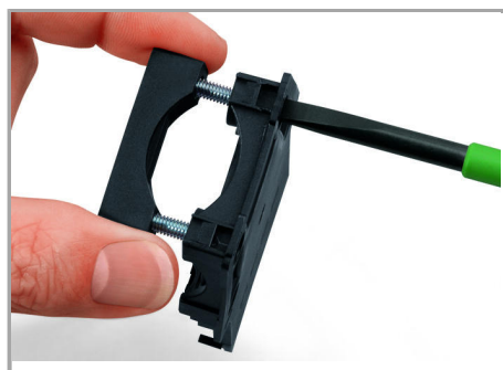
Unscrew base of strain relief housing.
