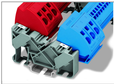
Busbar carrier (812-140):
