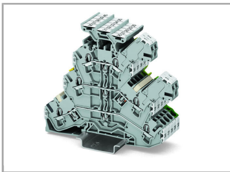
TOPJOB® S L-type test plugs for testing rail-mount terminal blocks via conductor entries
