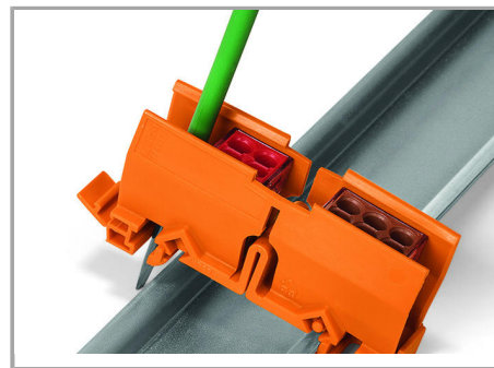
Remove the mounting carrier from the DIN-rail.
