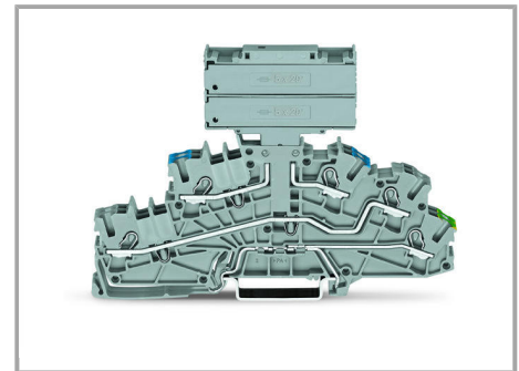
Double-fuse plugs with (5 x 25) mm miniature metric fuses can be used on carrier terminal blocks without N-knife disconnect in standard terminal block width.
