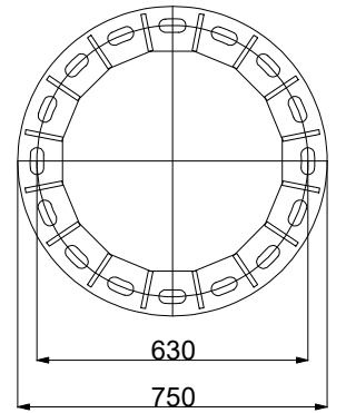
BASE PLATE Ø750x20mm
